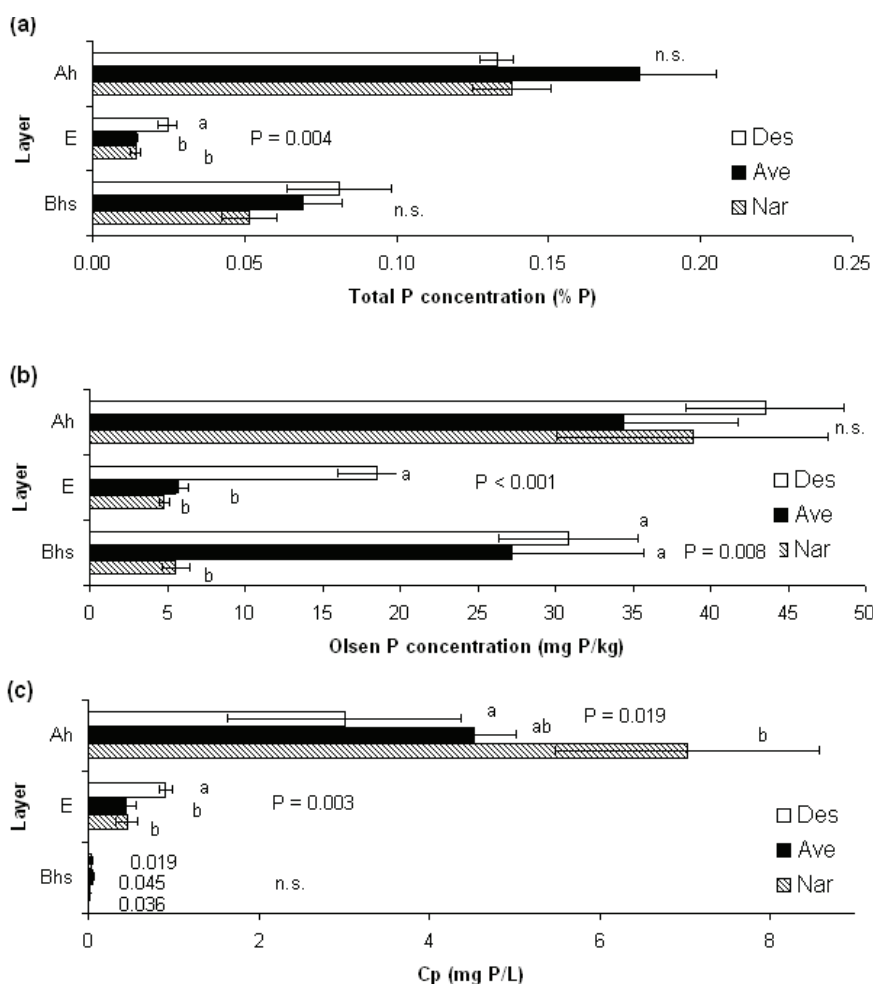
Fig. 2. (a) Concentration of total P, (b) Olsen P, and (c) Cp in 0–5 cm humus (Ah), 5–10 cm elluvial (E), and 20–30 cm illuvial (Bhs) soil layers; Areas abbreviations: Des = formerly fertilized dominated by D. cespitosa , Ave = transition zone dominated by A. flexuosa , Nar = unfertilized control dominated by N. stricta ; P = probability value obtained by One Way ANOVA analysis, n.s. = non-significant result of ANOVA, using Tukey's post hoc test; areas with the same letter are not significantly different; error bars represent standard error
